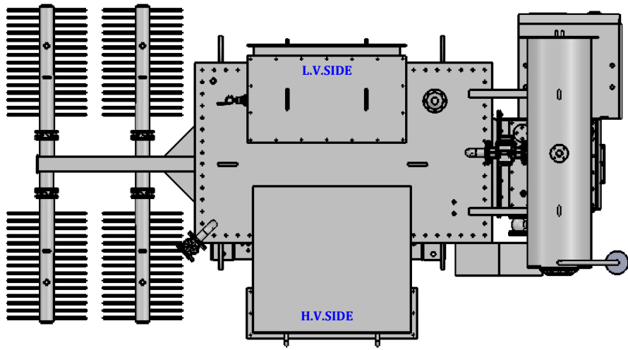
TOP VIEW
